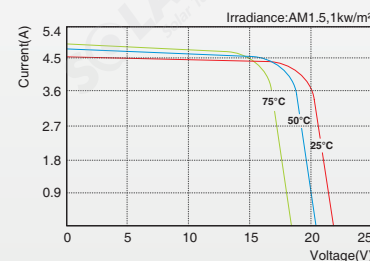
SLP070-12M I-V Curves
